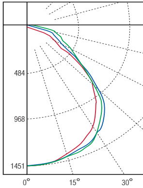
Candela Plot 2 Lamp T8
