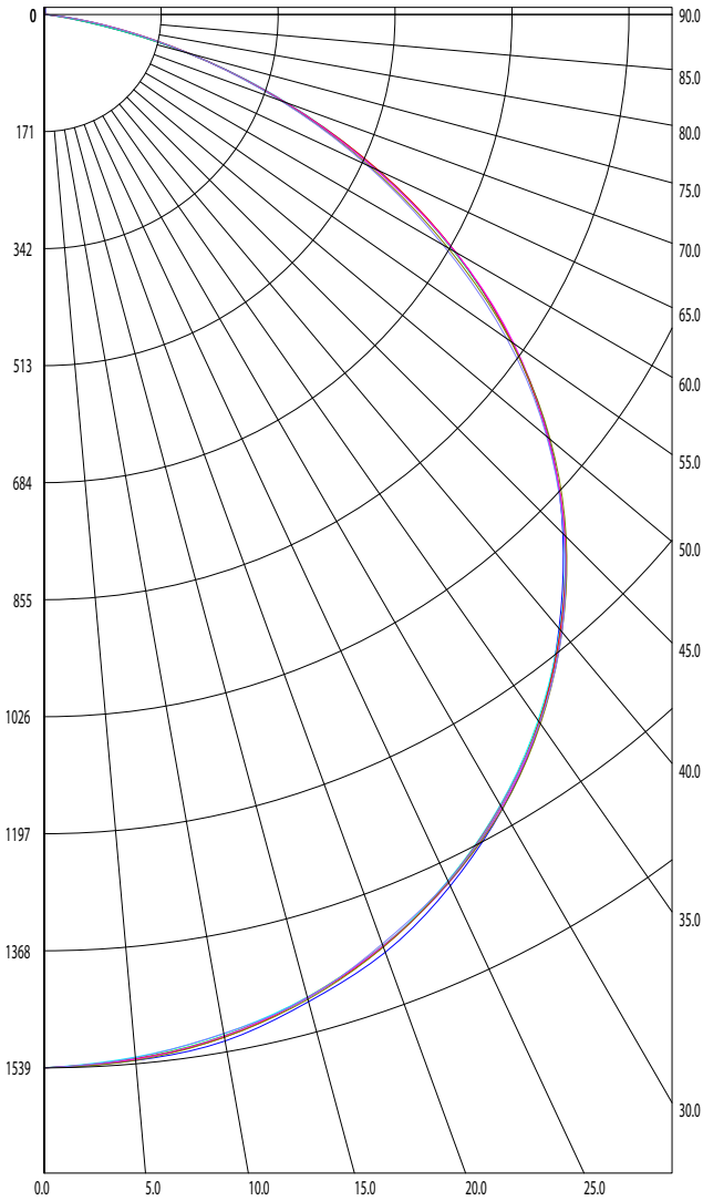
Luminaire Classification System Plot
